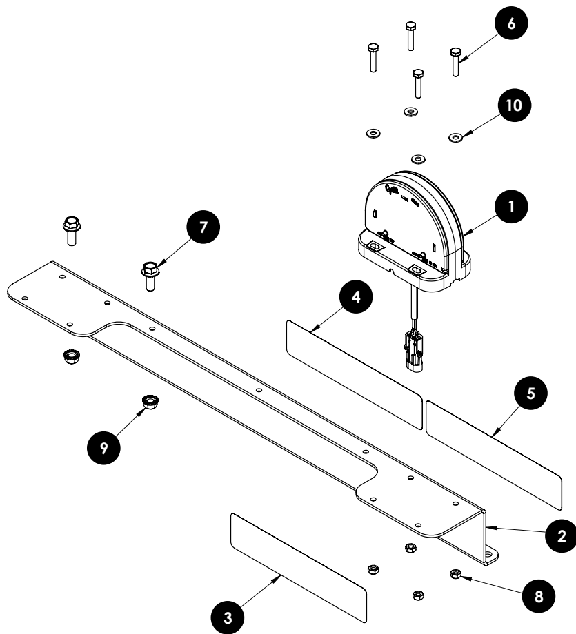
103295 HARNESS, ELEC., LIGHT SOCKET, TOWABLE CART
